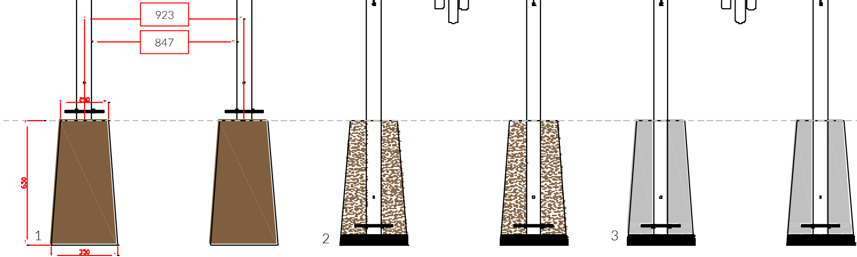
Excavate 2 holes with a 250mm diameter tapering down to 150mm diameter and 600mm depth 600mm min depth- Max Depth 1200mm
